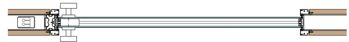
Puerta corredera Flat Door - Duo10 con hoja de 2 vidrios enmarcados Porta corredeira Flat Door - Duo10 com folha de 2 vidros encaixilhados Sliding door, Flat Door - Duo10 with double-glazed leaf, alum. frame Porte coulissante Flat Door - Duo10 avec panneau de double vitrage
